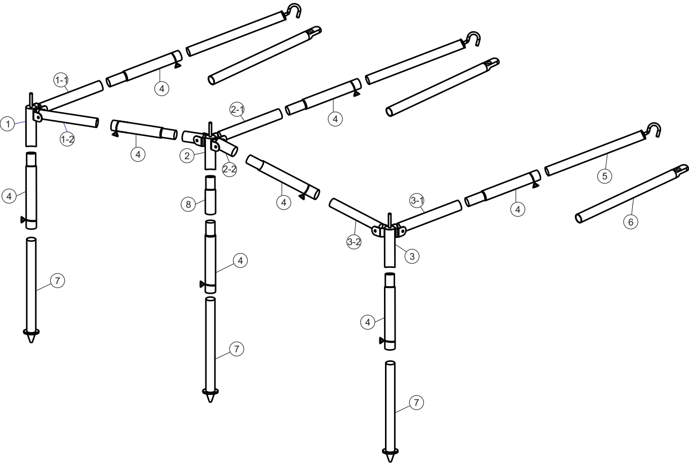
List of assembling parts
